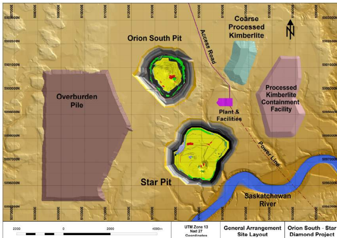
Figure 18-2: Site Layout
