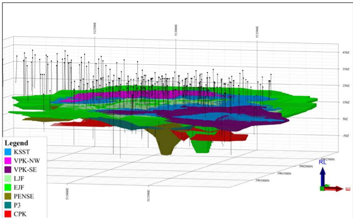
Figure 7-15: 3D View of the Orion South Kimberlite Geological Model Looking North West
