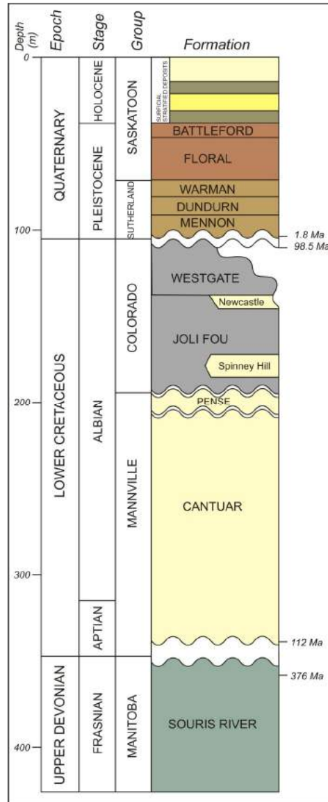
Figure 16-3: Overburden Stratigraphy
