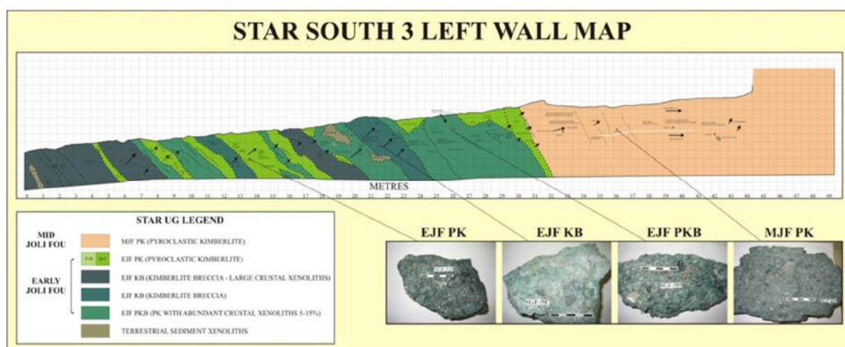
Figure 11-1: Example of an Underground Wall Map Showing the Contact between the Bedded EJP (Shades of Green) Kimberlite and the More Massive MJF Kimberlite (Peach)
