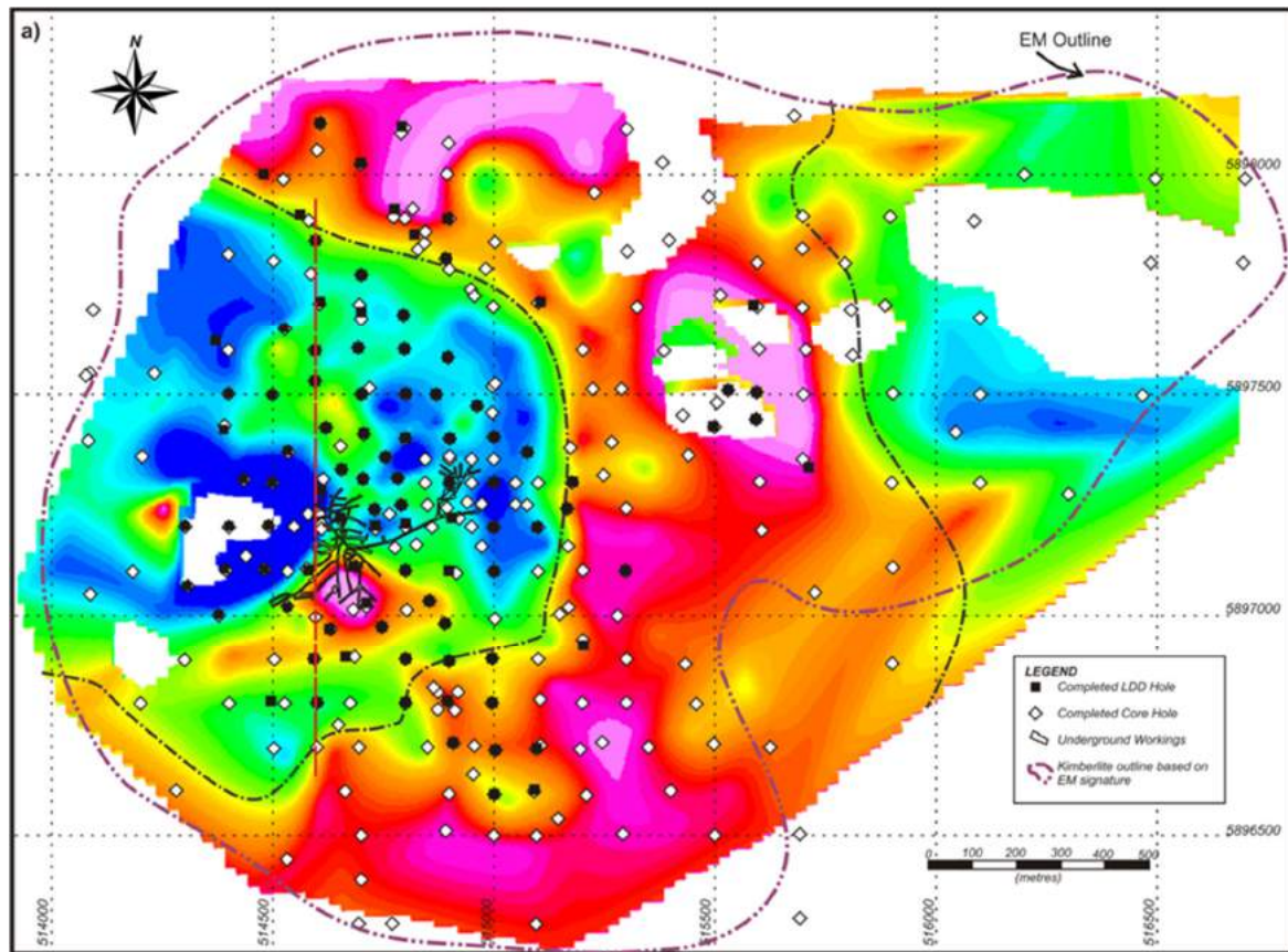
Figure 7-5: Topographic Elevation Map (Lows are Blue; Highs are Magenta) of the Top Contact of the Olivine Rich EJV
