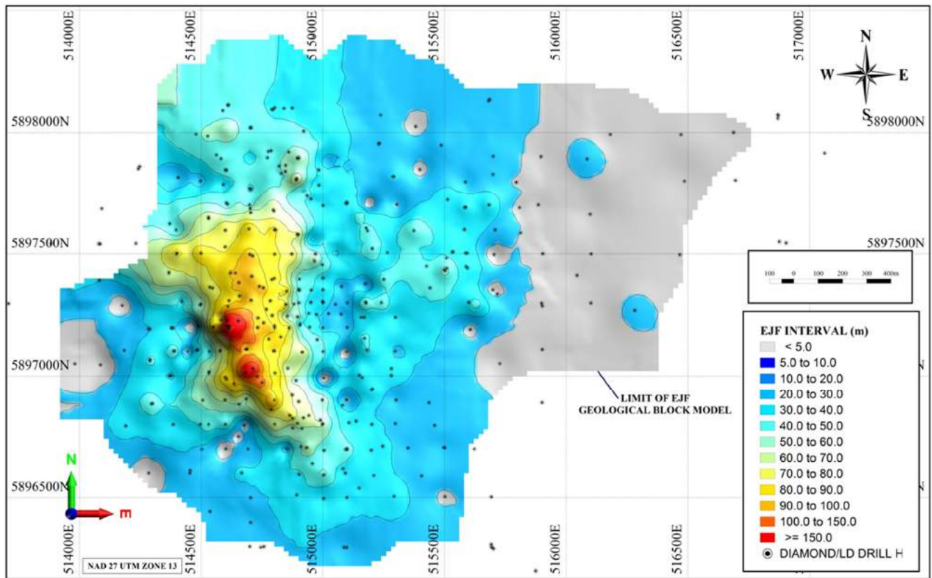
Figure 7-6: Isopach Map of the EJV Kimberlite Intersections (Contour Interval : 10 m)
