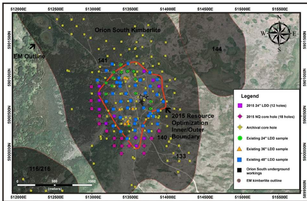
Figure 10-2: Drilling Map for the Orion South Kimberlite Deposit Including Core, Mud Rotary and Large-Diameter Drilling
